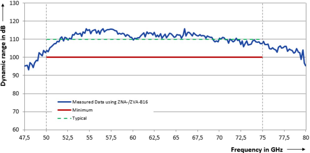
Dynamic range versus frequency of the R&S®ZC75
