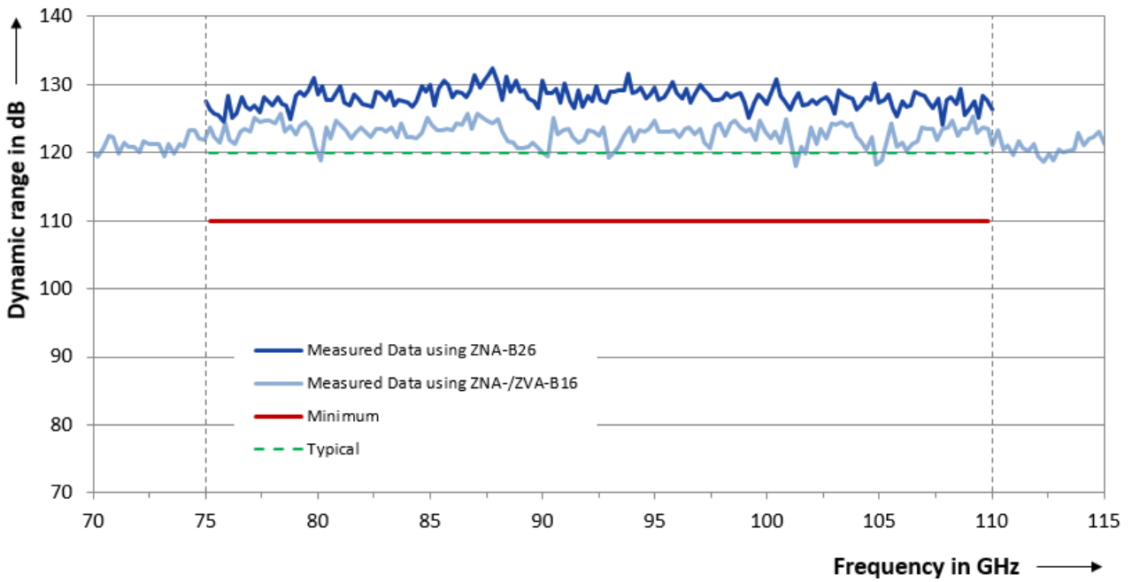
Dynamic range versus frequency of the R&S®ZC110
